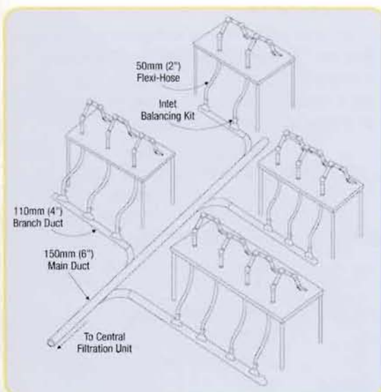
Typical ducting installation using articulated arms
